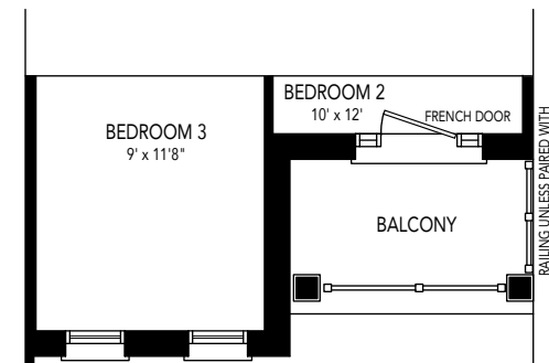
PART. SECOND FLOOR PLAN - ELEV. 'B'
