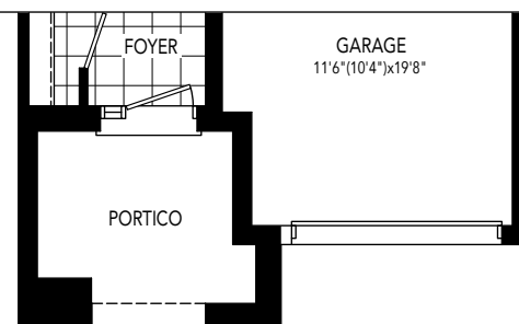
GROUND FLOOR PLAN - ELEV. 'A1' & 'B1'
