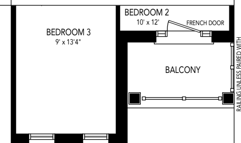
PART. SECOND FLOOR PLAN - ELEV. 'B1'
