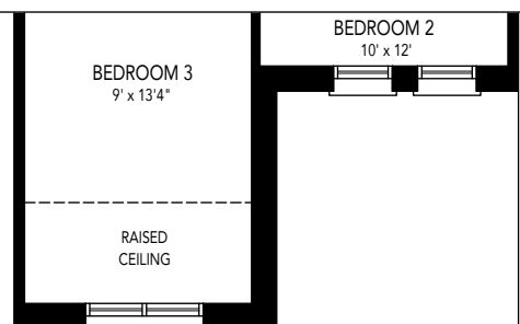
SECOND FLOOR PLAN - ELEV. 'A1'
