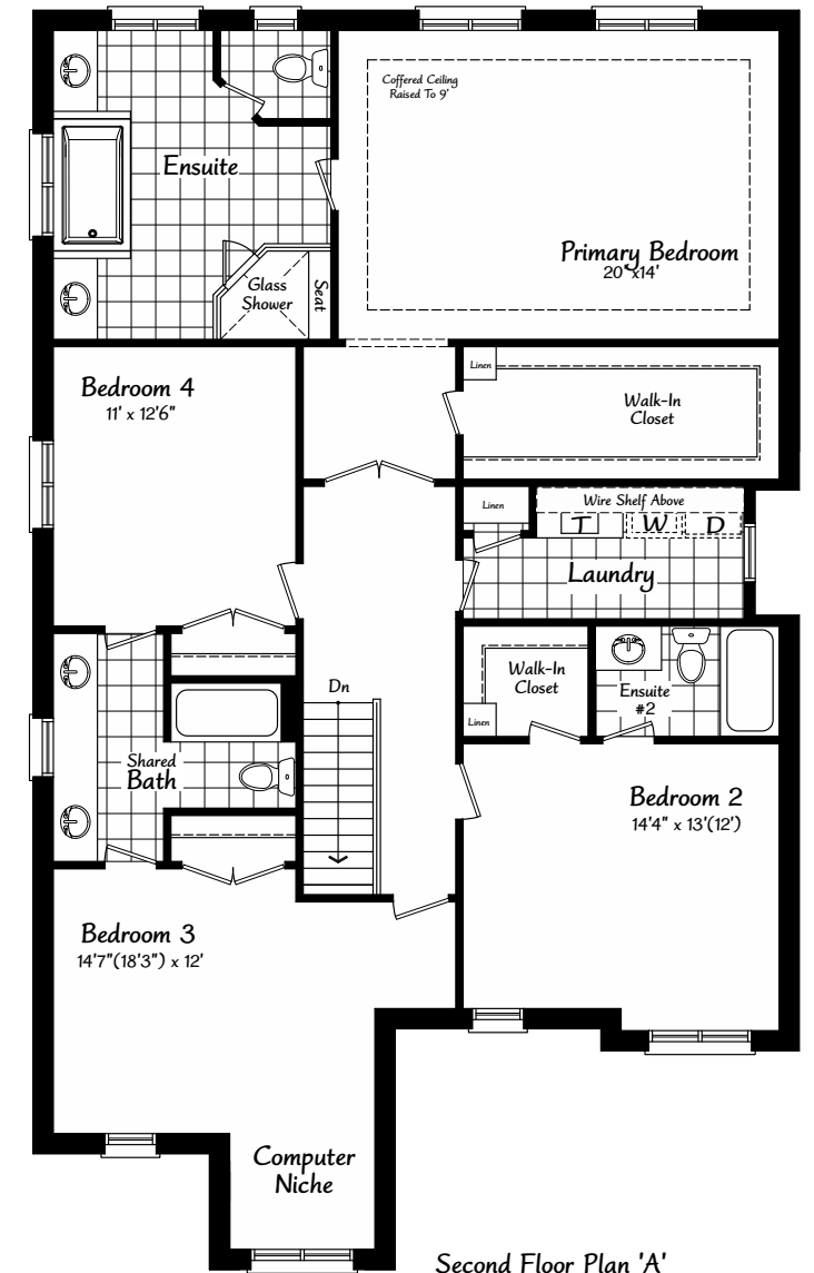
Second Floor Plan 'A'
