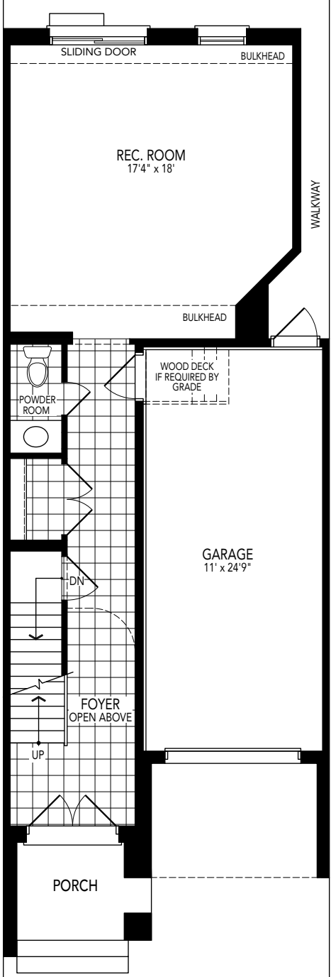
GROUND FLOOR PLAN ELEVATION 'A' & 'B'
