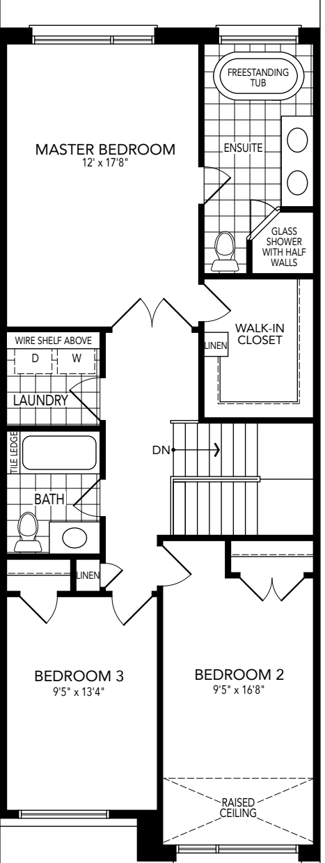
THIRD FLOOR PLAN ELEVATION 'A'
