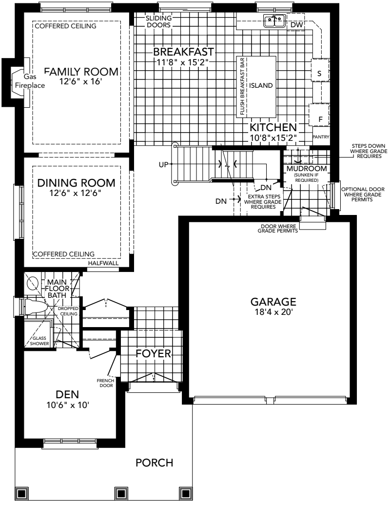
GROUND FLOOR PLAN ELEVATION 'A'
