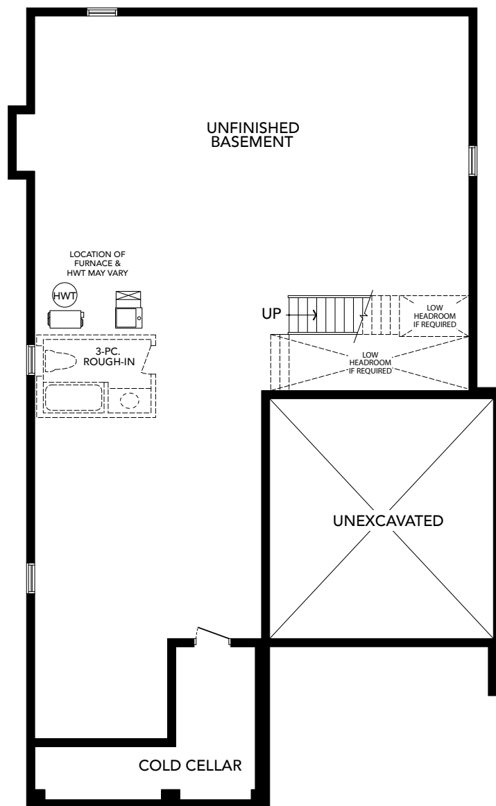
BASEMENT PLAN ELEVATION 'A'
