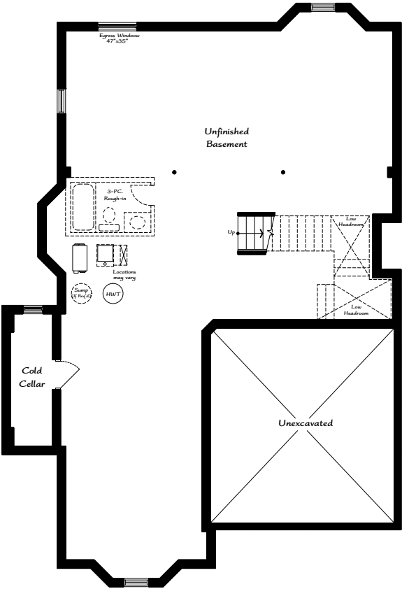
Basement Plan 'A'
