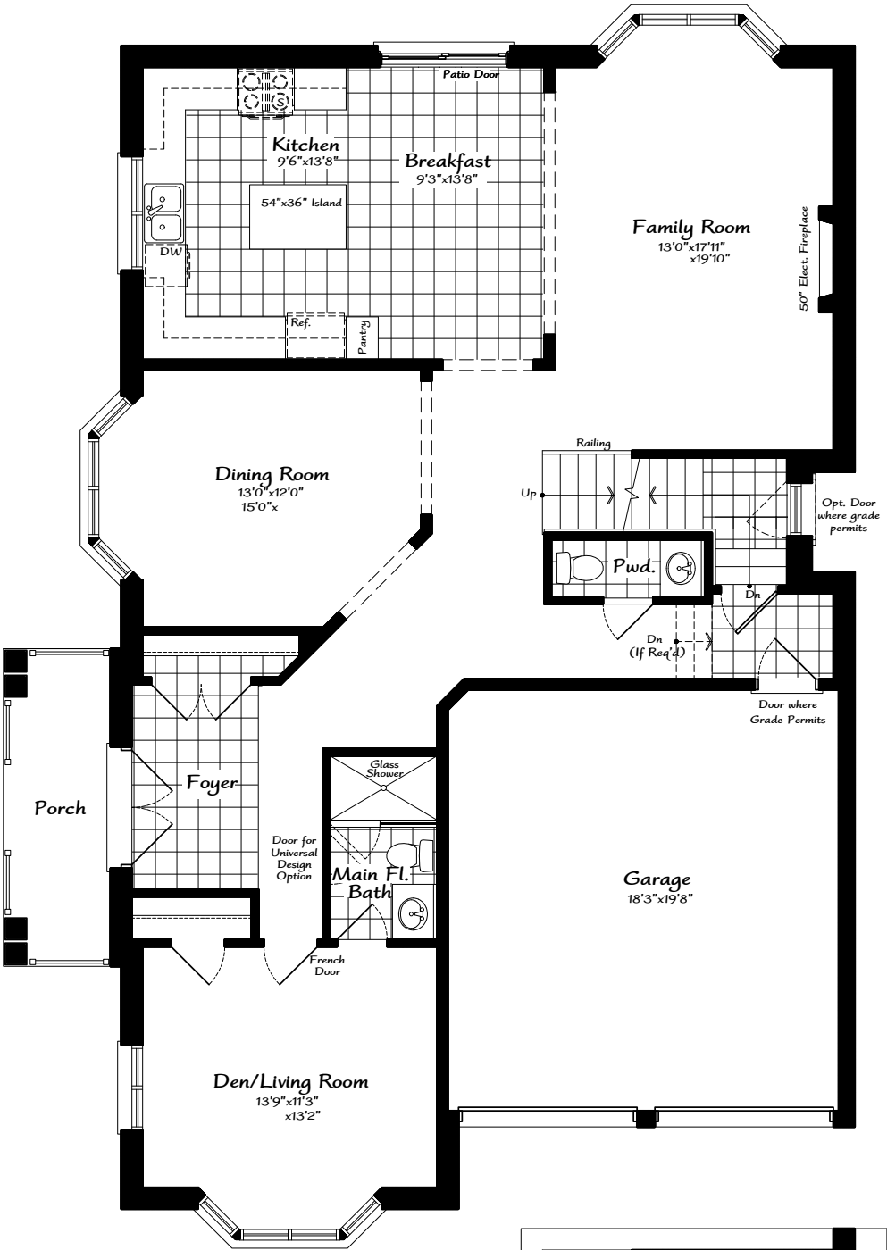
First Floor Plan 'A'
