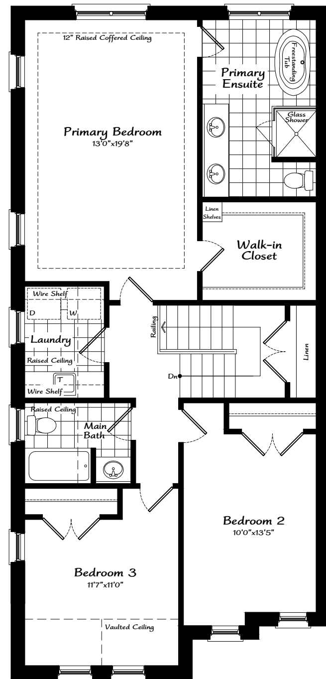
Second Floor Plan 'A' 3 Bedrooms
