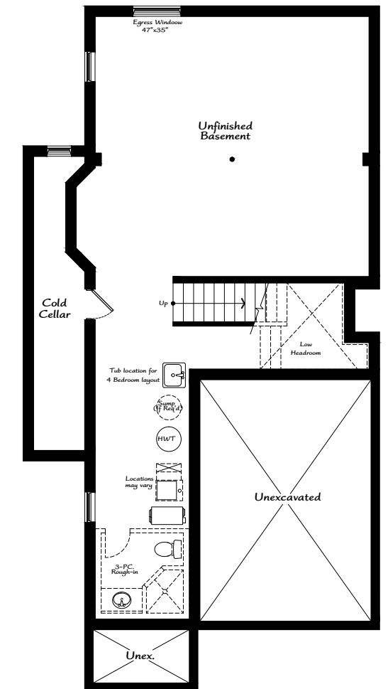
Basement Plan 'A'
