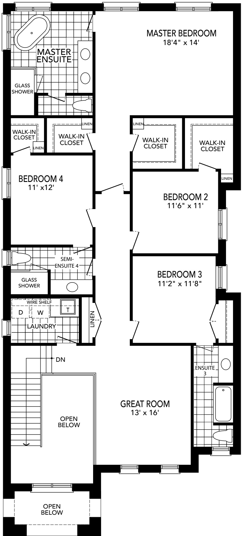
SECOND FLOOR PLAN 4 BEDROOM ELEVATION 'A'
