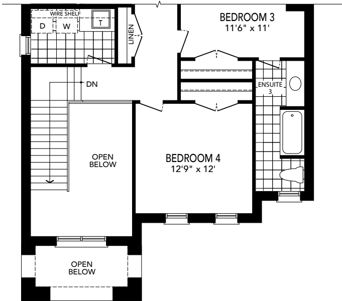
OPTIONAL SECOND FLOOR PLAN ELEVATION 'A' 5 BEDROOM IN LIEU OF GREAT ROOM
