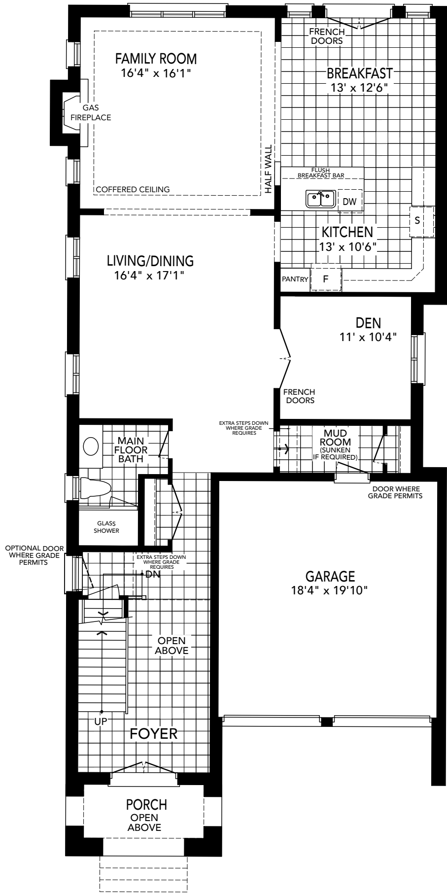
GROUND FLOOR PLAN ELEVATION 'A'
