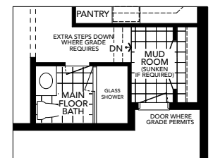
PARTIAL GROUND FLOOR PLAN FULL BATH
