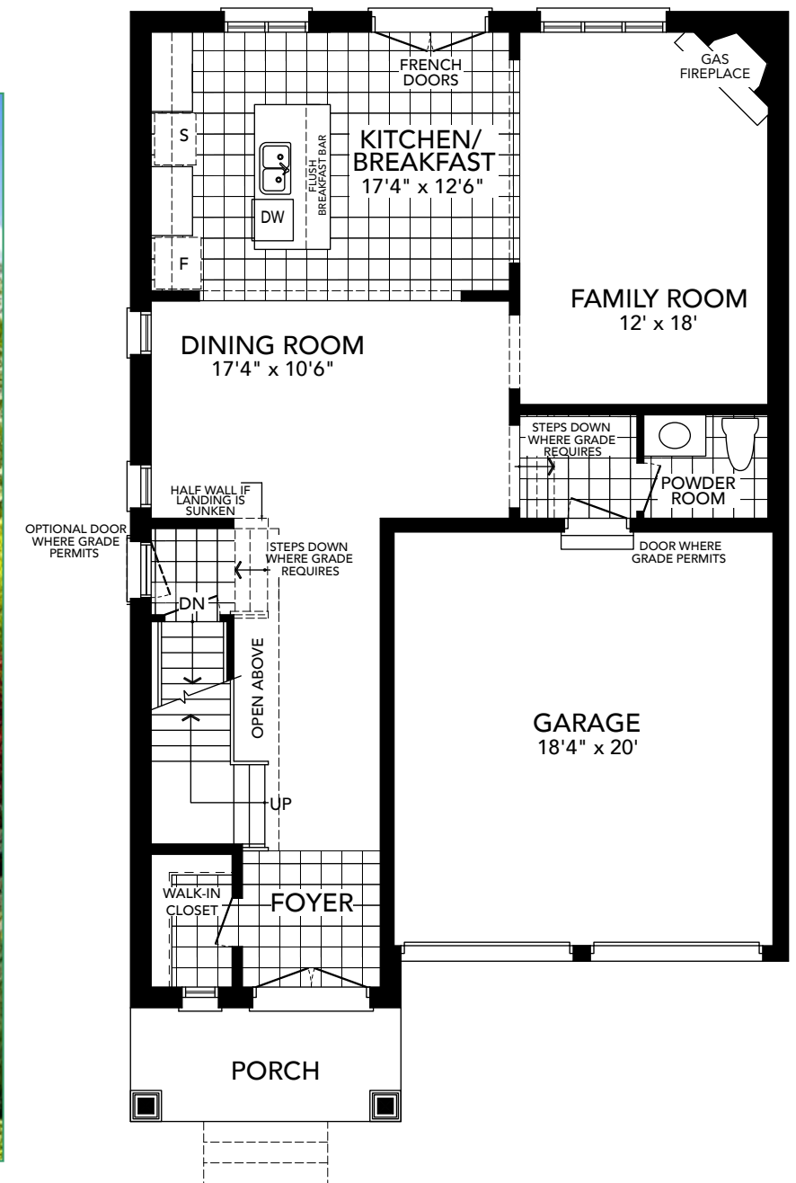
GROUND FLOOR PLAN ELEVATION 'A'
